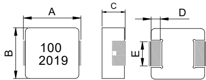
leadframe
