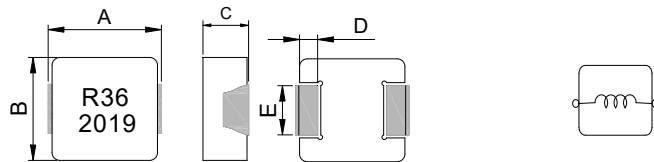
non-leadframe
